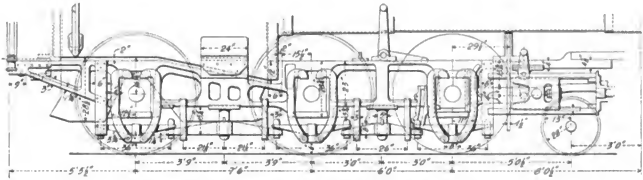
Fig. 1654. Spring Rigging for Ten-Wheel (4-6-0) Locomotive.
